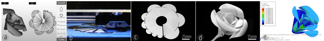
Figure 1. Thermorph overview. (a) Design editor to define and simulate the self-folding composite; (b) the printing toolpath of a flat sheet is generated from (a) and printed on an FDM printer; (c) the printed flat sheet; (d) the flat sheet self-folds sequentially into a rose; (e) finite element based simulation of the self-folding rose to verify our hypothesis on the material mechanism.
