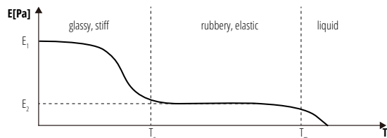
Figure 3. State transitions of thermoplastics: stiffness versus heating temperature.
